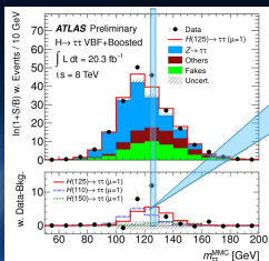
Evidence for Higgs Boson Decays to the \tau^+ \tau^- Final State with the ATLAS Detector ATLAS-CONF-2013-108 (28 November 2013)
